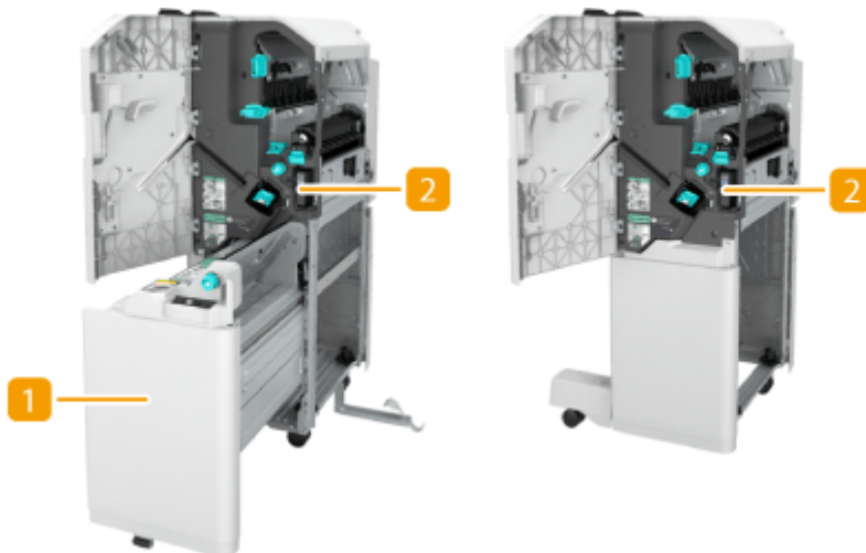
Booklet Finisher-V
